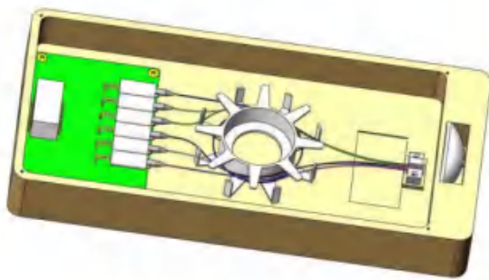
TX Transmitter Optical Module( Solution 1)
